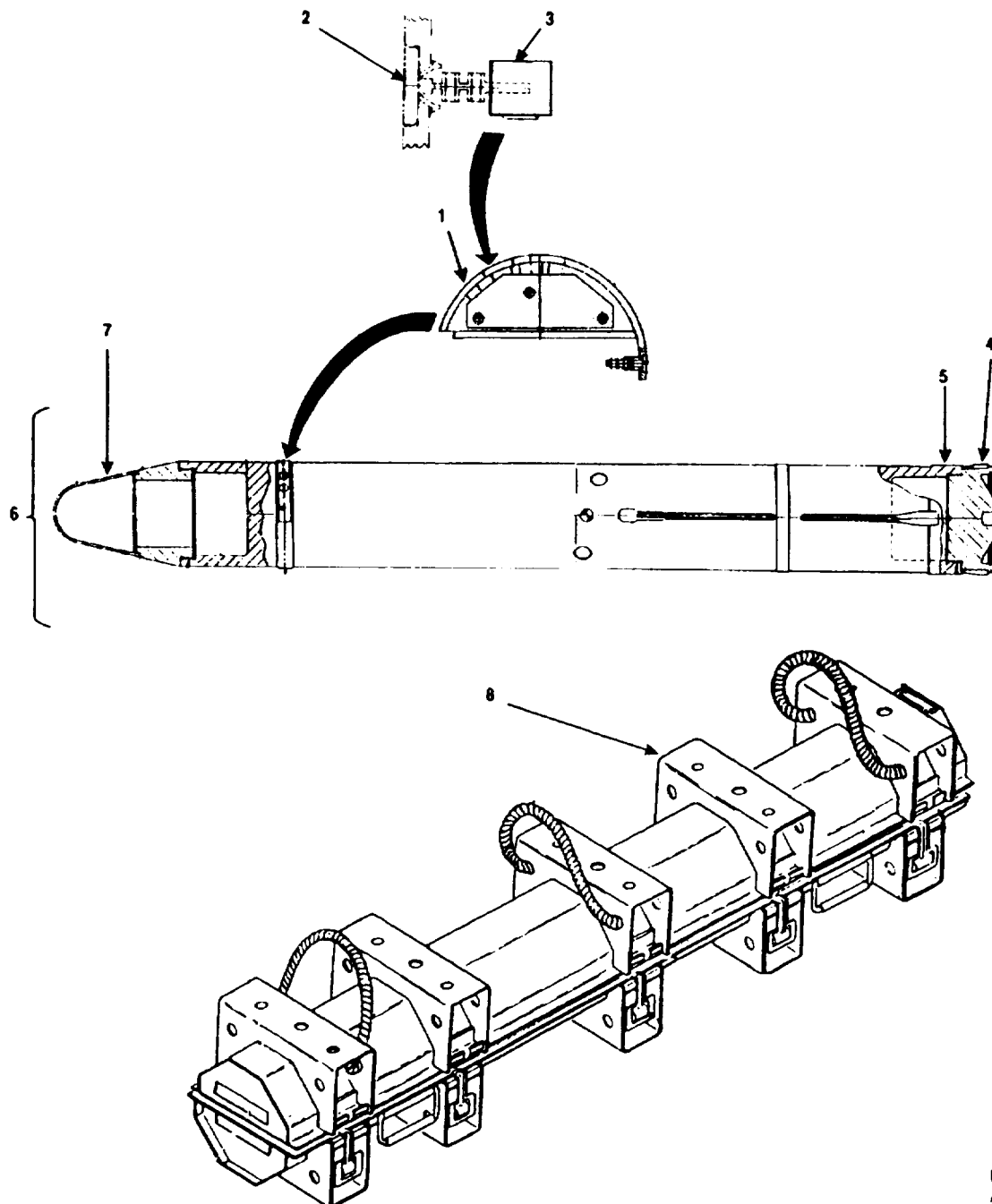
FIGURE C1. PROJECTILE, 155MM:
